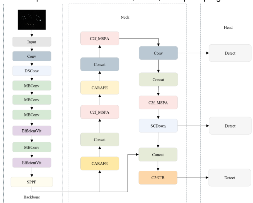
Fig. 3 – The network structure of EMC-YOLO
