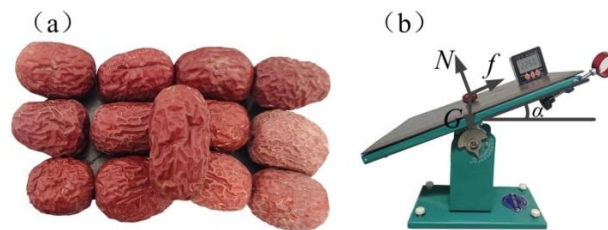
Fig. 1 - Measurement of the static friction coefficient (a) Jujube contact surface; (b) Inclined-plane test setup
