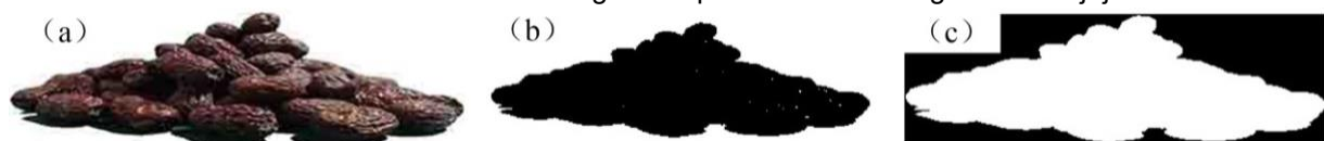
Fig. 3 - Image-processing procedure for determining the angle of repose (a) Original image; (b) Morphological processing; (c) Contour extraction and fitting
