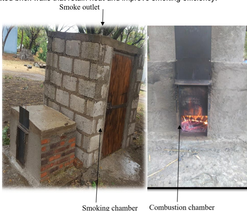
Fig. 4 - Stationary or fuelwood fish smoking technology
