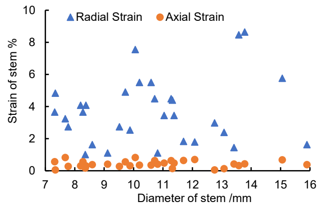
Fig. 6 - Effect of diameter on tensile strain
