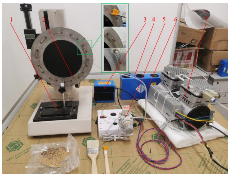
Fig. 1 - Experimental setup for the single-factor test of the seed metering plate
