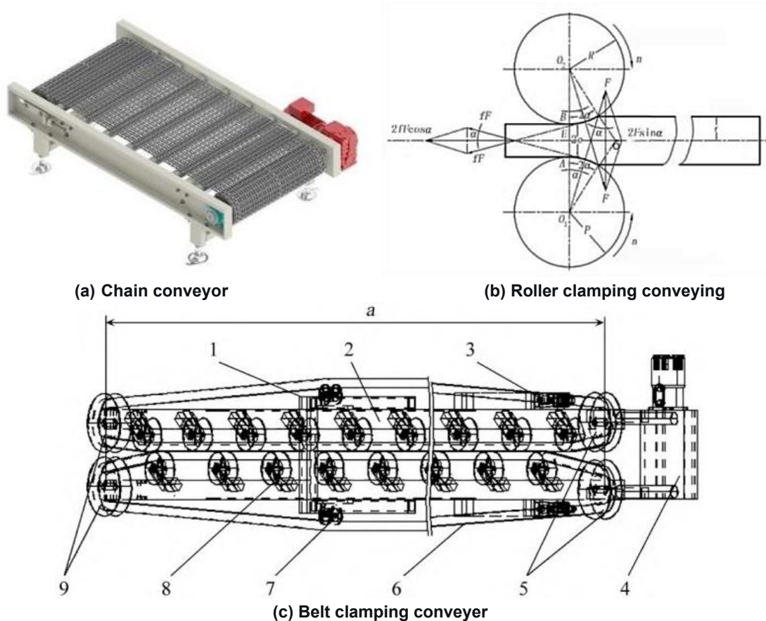
Fig. 5 - Transport Device
