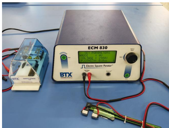
Fig. 3 - High voltage pulsed electric field treatment device
