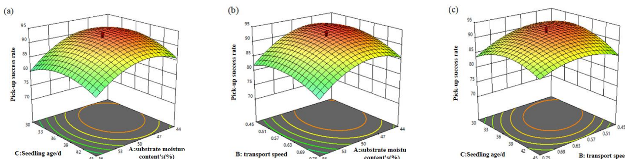
Fig. 12 – The influence of experimental factors on the success rate of taking and throwing seedlings
