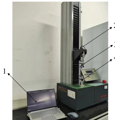
Fig. 3 - Mechanical properties test instrument
