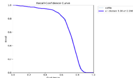
Fig. 12 - Recall-Confidence
