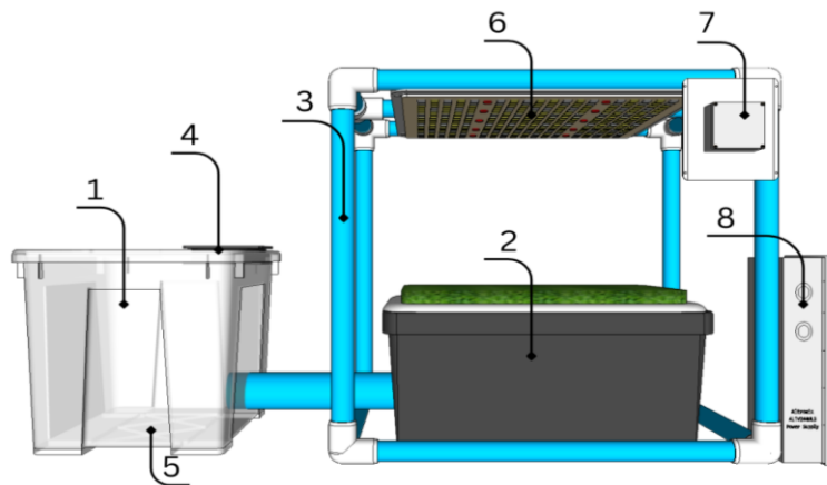
Fig. 1 - Fogponics system setup 1 - nutrient tank, 2 - seedling box, 3 - main frame, 4 - fan, 5 - ultrasonic fogger, 6 - LED light, 7 - control system, 8 - power supply
