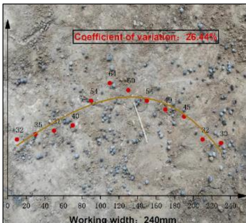
Fig. 10 - Top view of particle distribution
