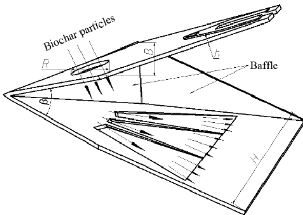
Fig. 2 - Trenching and return shovel
