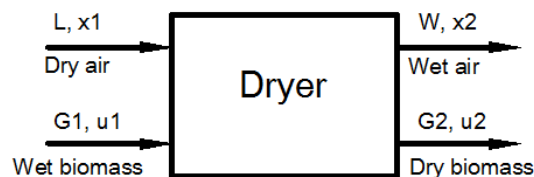
Fig. 1- Block diagram of the artificial drying process
