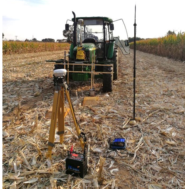
Fig. 4 - Field profiling validation test
