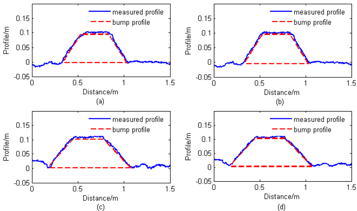
Fig. 9 - Measured profiles in one of the field profiling validation tests
