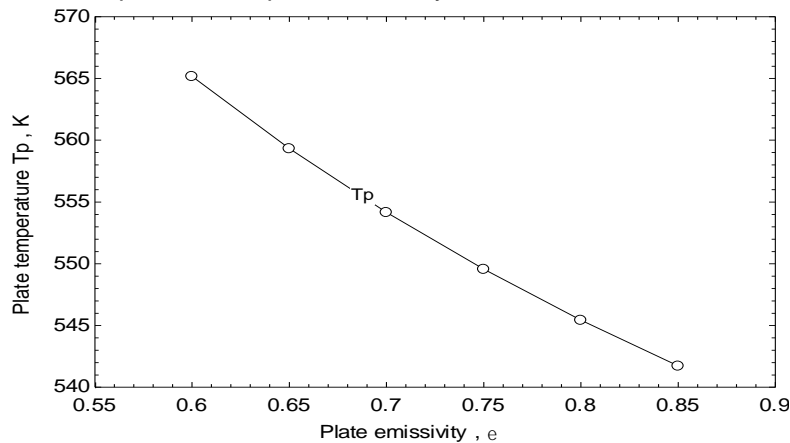
Fig. 5 - Variation of plate temperature with Plate emissivity
