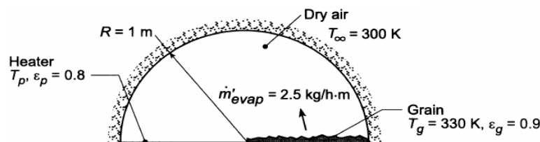
Fig. 2 - Analysis of the semi-circular grain dryer
