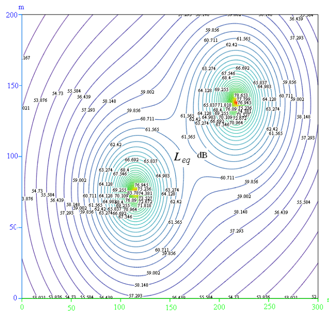
Fig. 15 - The noise field generated by two working Bulgarian tractors in a field of 200 x 300 m size The first (right) tractor works at 2000 RPM, and the second (left) at 1500 RPM
