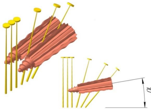
Fig. 7 - Scheme for capturing and transporting stems by rotor
