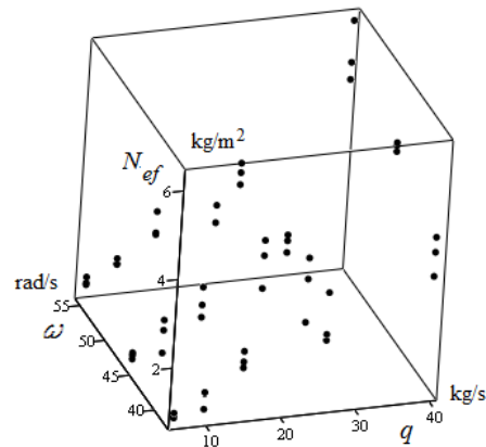
Fig. 4 - Distribution of effective norm values (interpolated variant) in relation to material flow and rotation speed of rotors
