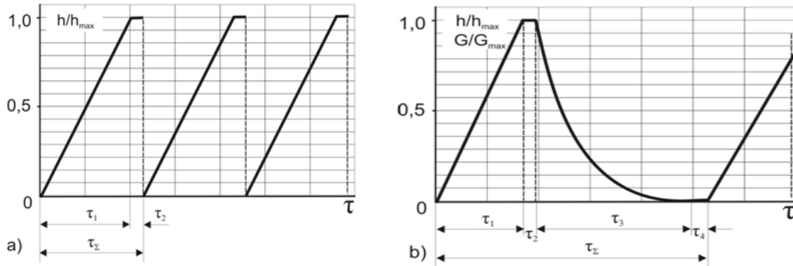
Fig. 1 - Operation cyclograms of discrete action dosimeters
